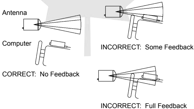
Figure 8.2.5 Correcting feedback interference.
