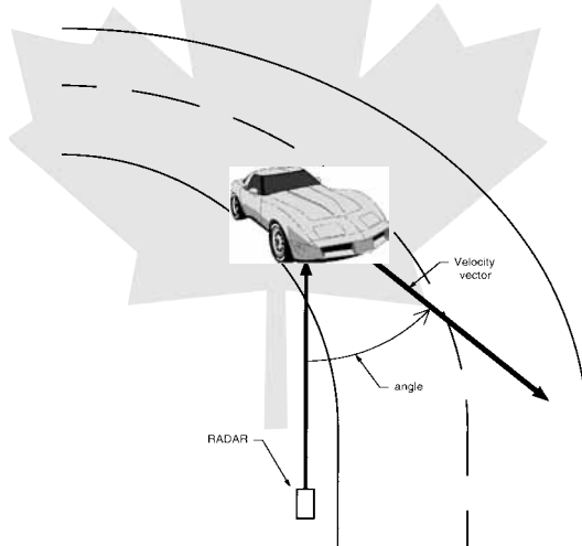
Figure 8.2.1 An angle between the antenna and the target vehicle causes the cosine effect.
