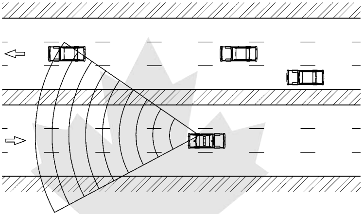
Figure 3.4a A patrol vehicle that is tracking a target vehicle with the rear antenna while traveling with the radar unit in Moving Mode Opposite Direction.
