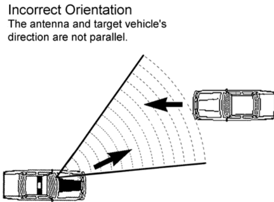
Figure 2.3c Orientation of the antenna to the target vehicle.
