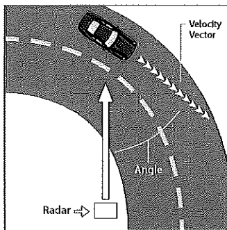
Figure 7.2.1a An angle between the antenna and the target vehicle causes the cosine effect.
